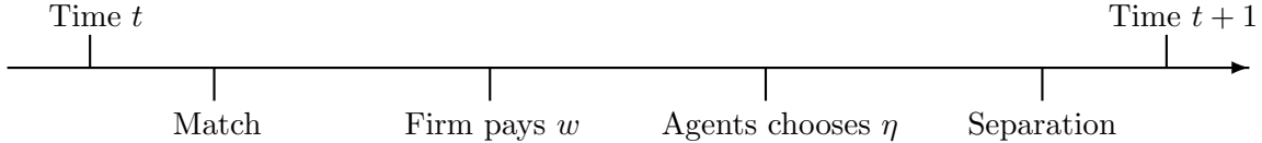
Figure 2: Timeline of Period t .
