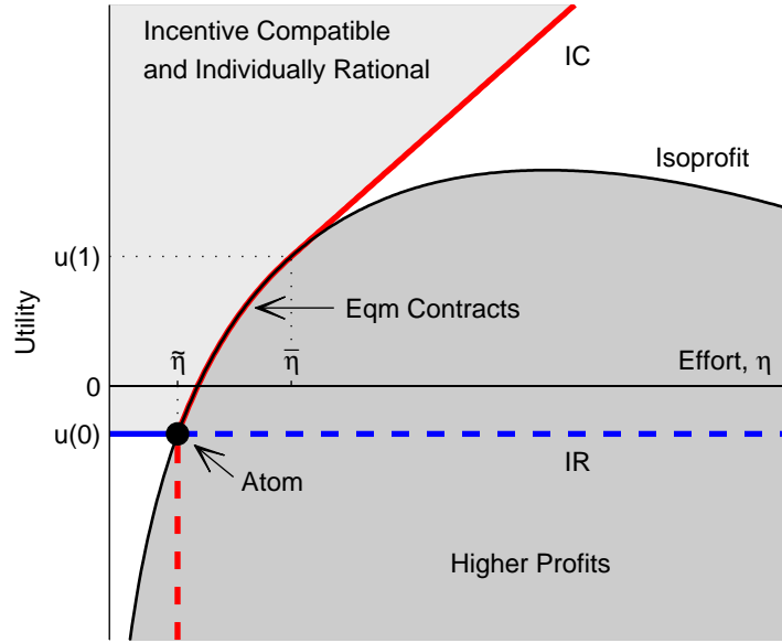
Figure 5: The Set of Optimal Contracts with Intern Matching. This figure shows the firm’s isoprofit curve u = \phi(\eta) - \eta - \pi , the worker’s IC constraint u_*(\eta) , and the IR constraint for the equilibrium contracts. Firms x \geq \tilde{x} have effort satisfying the first-order condition; firms x \leq \tilde{x} offer the contract \langle u(0), \eta(0) \rangle = \langle -\tilde{\eta}, \tilde{\eta} \rangle which pays wage w(0) = 0 .
