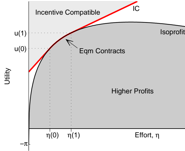
Figure 3: The Set of Equilibrium Contracts. This figure shows the firm’s isoprofit curve u = \phi(\eta) - \eta - \pi and the worker’s incentive compatibility constraint u_*(\eta) in equilibrium. Contracts under the isoprofit line are more profitable for the firm; contracts above the IC constraint are incentive compatible. When solving for equilibrium, the firm’s first-order condition says the isoprofit curve must be tangent to the IC constraint; profits are determined so these curves coincide over the range of equilibrium contracts.
