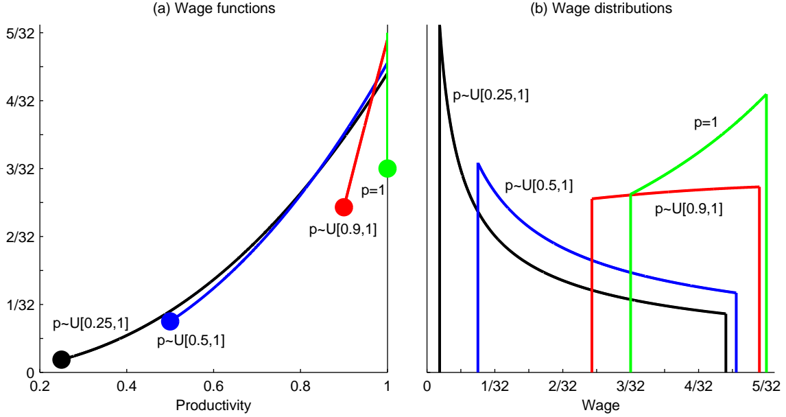
Figure 6: Wages with Heterogeneous Firms. This figure shows wages for p \sim [0.25, 1] , p \sim [0.5, 1] , p \sim [0.9, 1] and p = 1 . Panel (a) shows the wage function w(p) , while panel (b) shows the resulting densities of wages. This figure assumes output is \phi(\eta, p) = p\sqrt{2\eta} , the mass of firms is n = 2/5 , the breakup rate is 1 - \alpha = 1/2 , and the discount rate is \delta = 1/2 .
