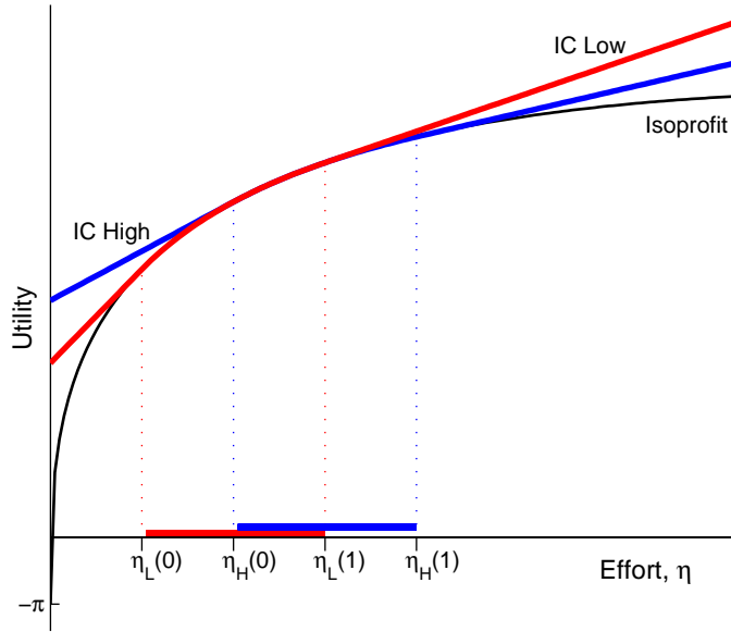
Figure 7: Equilibrium Effort and Wages with Heterogeneous Workers. This figure illustrates the equilibrium effort ranges for low-type and high-type workers. Moving along the isoprofit curve, worker \kappa 's IC constraint is satisfied with equality for \eta \in [\eta_\kappa(0), \eta_\kappa(1)] and violated for other effort levels.
