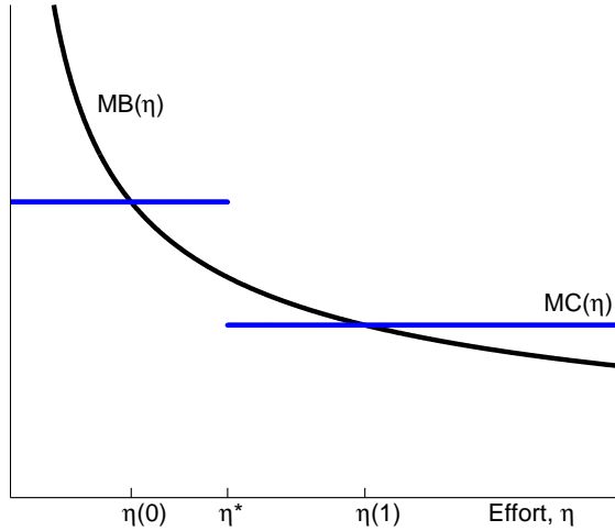
Figure 1: Impossibility of Single-Wage Equilibria with On-the-Job Search. This figure illustrates the marginal benefit and cost of effort for a single firm when all other firms offer the same contract \langle w^*, \eta^* \rangle . Turnover and the marginal cost of effort are discontinuous at \eta^* while the marginal benefit of effort is continuous. Thus, MB < MC just below \eta^* yielding a profitable downward deviation; similarly, MB > MC just above \eta^* yielding a profitable upward deviation. More generally, one or other of these deviations is profitable for any value of \eta^* .
