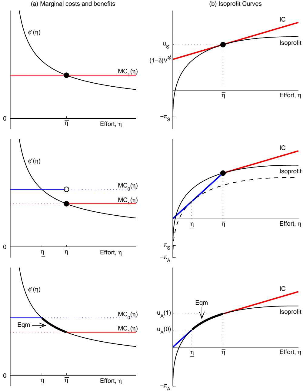
Figure 4: The Impact of On-the-Job Search. The top left panel illustrates the marginal benefit and marginal cost of effort MC_1(\eta) under Shapiro-Stiglitz matching when other firms offer the Shapiro-Stiglitz equilibrium contract with effort \bar{\eta} . The top right panel shows the firm's isoprofit function and the worker's IC constraint. The middle panels introduce anonymous matching and suppose other firms continue to offer the Shapiro-Stiglitz contract. When the firm offers a lower wage, it faces a lower retention rate and higher marginal cost of effort MC_0(\eta) , but does not need to compensate its worker for the opportunity cost of forgone searching, (1 - \delta)V^\varnothing . This yields a profitable deviation with effort \underline{\eta} . The bottom panels show the equilibrium under anonymous matching. Here, MC_1(\eta) and MC_0(\eta) are marginal costs for highest and lowest firms (i.e. quantiles 1 and 0). The distribution of contracts is determined so that each firm equates the marginal cost and benefit of effort, and achieves the same profit.
