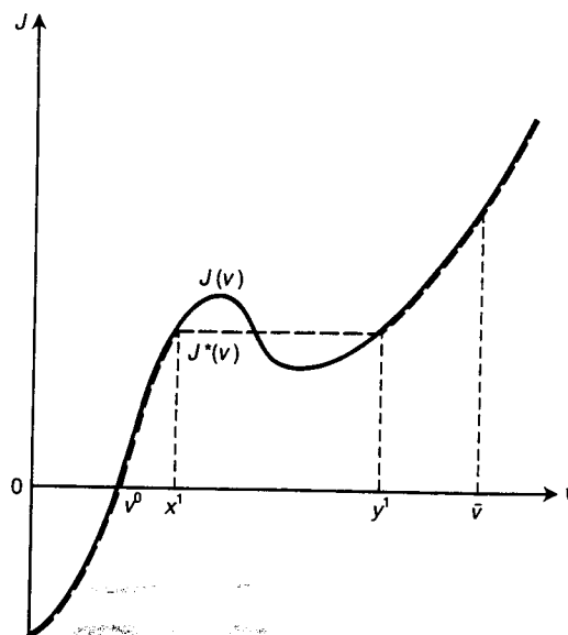
Fig. 14.1 Derivation of J^* .
